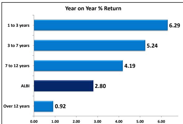
Year on Year the All Bond Index was Up (2.8%) The Highest Yield was 1 to 3 years (6.29%)
