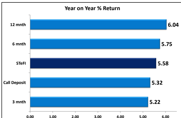
Year on Year the STeFI Index was Up (5.58%) The Highest Gain received - the 12 mnth (6.04%)
