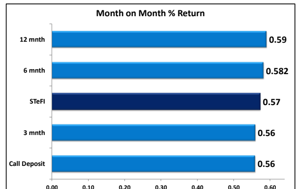
Month on Month the STeFI Index was Up (0.57%). The Highest Gain received - 12 mnth (0.59%)
