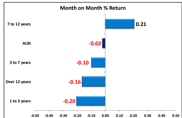
Month on Month the All Bond Index was Down (-0.02%) The Highest Yield was 7 to 12 years (0.21%)
