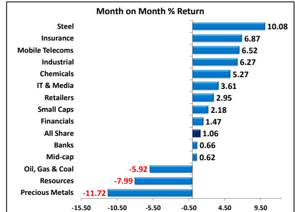
Month on Month - JSE All Share Index was Up (1.06%) The Best Performer was Steel (10.08%)
