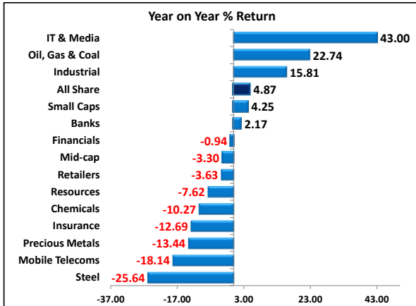
Year on Year the JSE All Share Index was Up (4.87%) The Best Performer was IT & Media (43%)
